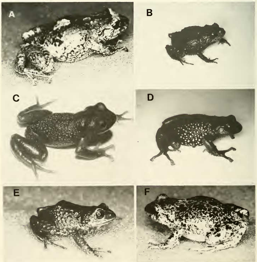
FIG. 12. Andean Eleutherodactylus . (A) E. modipeplus , KU 120021, 34.2 mm; (B) E. myersi , KU 168436, 18.9 mm; (C) E. orcesi , AMNH 104720, 32 mm SVL; (D) E. orcesi , KU 177814, 35.2 mm; (E) E. thymelensis , topotype, not preserved; (F) E. unistri-gatus , KU 119750, 28.4 mm.
